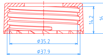
(38/400) CAP , P=1"x6 TPI
