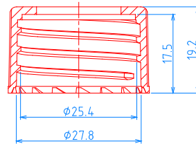
(28/415) CAP, P=1"x6 TPI
