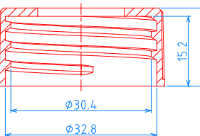
(33/410) CAP, P=1"x6 TPI
