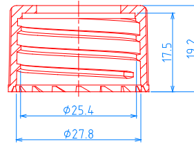
(28/415) CAP, P=1"x6 TPI
