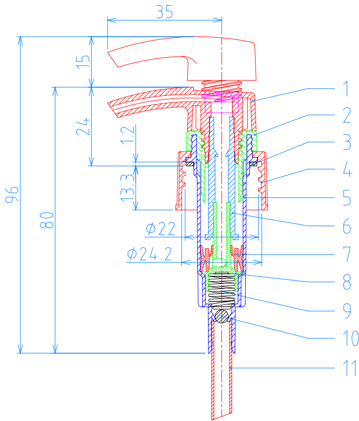
(28/410) CAP, P=1"x6 TPI
