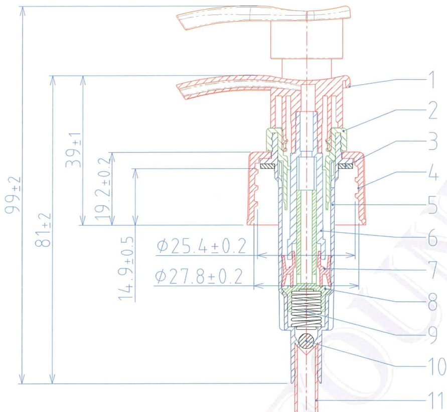
(28/415) CAP, P=1"x6 TPI
