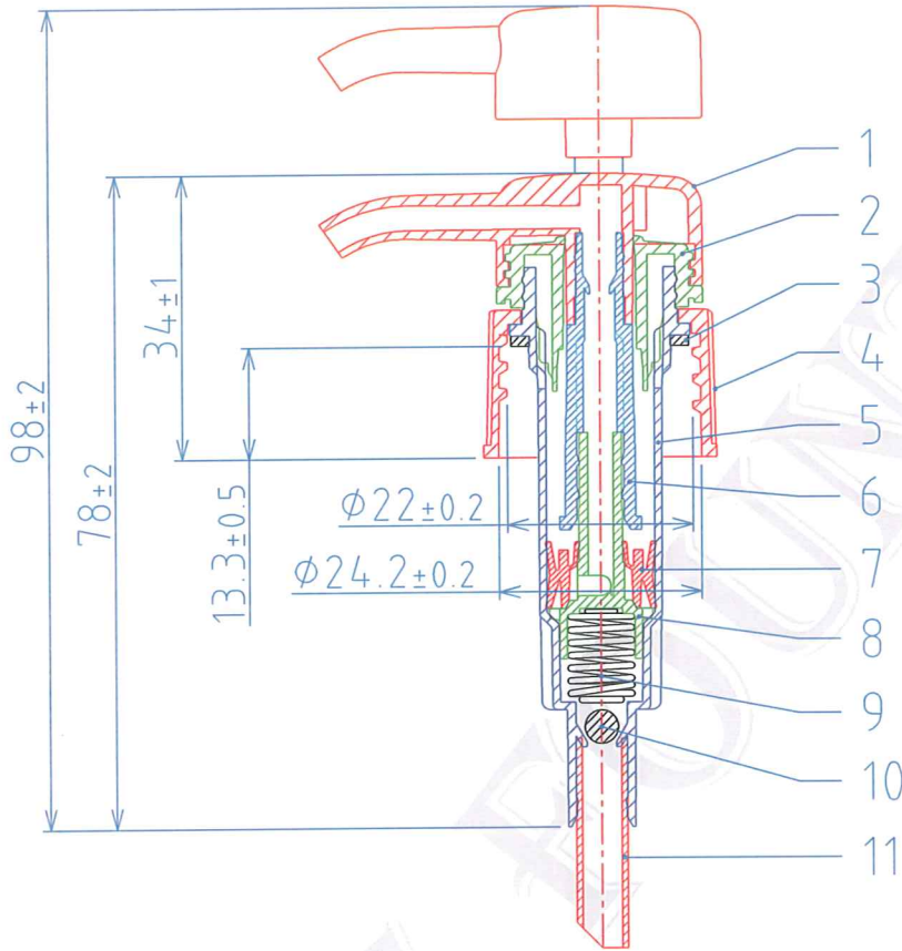
(33/410) CAP, P=1"x6 TPI
