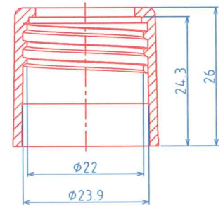
(28/400) CAP, P=1"x6 TPI
