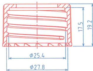
(28/410) CAP, P=1"x6 TPI
